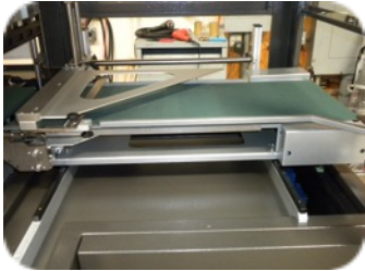
Motorized inverting triangle for package height adjustment
